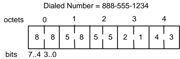
Figure 7: Sample DIALED NUMBER Encoding
