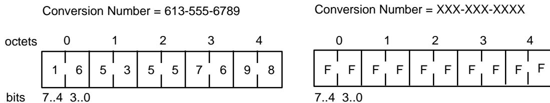
Figure 8: Sample CONVERSION NUMBER Encoding
