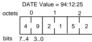
Figure 4: Sample DATE Value Encoding
