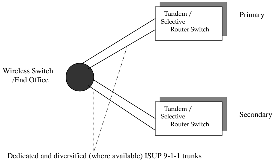
Figure 2: 9-1-1 Trunks
