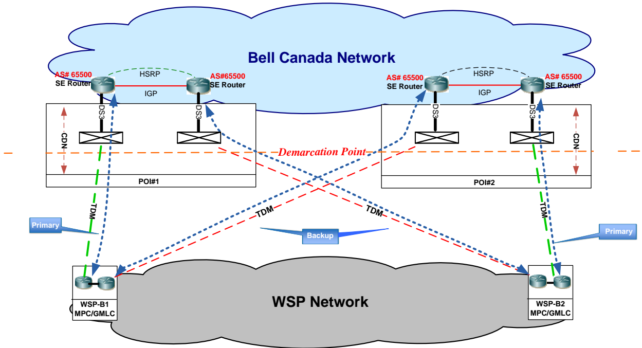
Figure 4: POI Interconnection for Remote Sites
